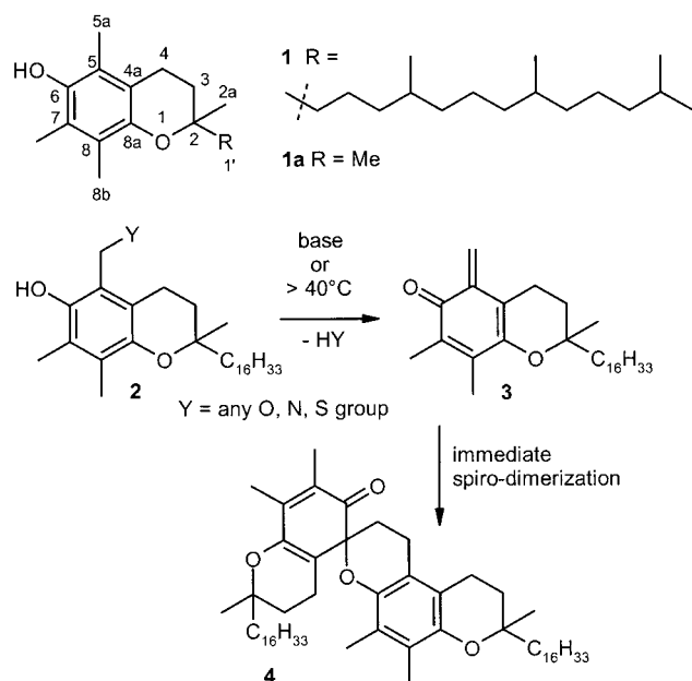
Scheme 1. Chemical behavior of 5a-substituted \alpha -tocopherols.
