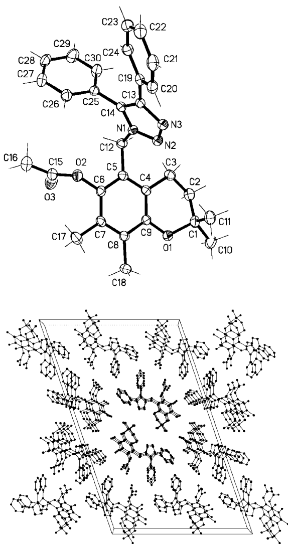
Figure 1. Thermal ellipsoid plot (40% ellipsoids), crystallographic atom labeling (top) and stacking plot along the b-axis (bottom) of tocopheryl-triazole 9 (4,5-diphenyl substituents).
