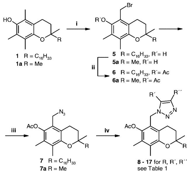
i: \text{Br}_2 , hexane, 120 min, r.t., quant.; ii: \text{Ac}_2\text{O}/\text{H}^+ , \text{CH}_2\text{Cl}_2 , 120 min, r.t. iii: \text{NaN}_3 , MeCN, 120 min, reflux, 84% for 7 from 5 ; iv: alkyne (up to 2.2 equiv.), toluene, reflux, 43–91% (see Table 1)
