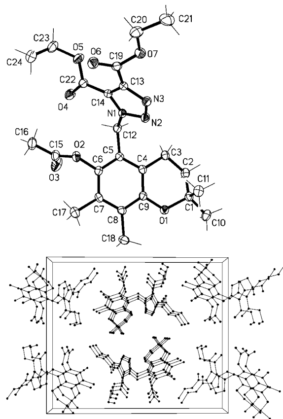
Figure 2. Thermal ellipsoid plot (20% ellipsoids), crystallographic atom labeling (top) and stacking plot along the a-axis (bottom) of tocopheryl-triazole 11 (4,5-diester substituents).
