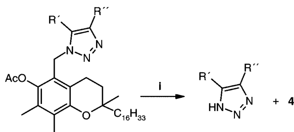
Scheme 3. Base-induced cleavage of the lipophilic 5a-tocopheryl moiety.
